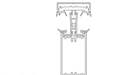
22 Fit hip and transom pressure plates by centralising, they will locate into the central channel on the rafter. Ensure that pressure plates are pushed up against the side of the ridge topcap.
