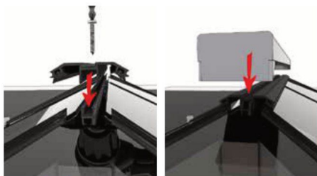
3 Fit ridge pressure plate and topcap.
