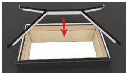
9 Position assembled frame onto ringbeam, pushing the hips down into place.
