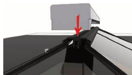
21 Fit the ridge top cap in place by centralising and applying pressure from one end to the other. A rubber mallet may be required.
