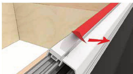
18 Peel back the corner of the glazing tape and remove.
