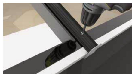
23 Screw down into the rafter through the pre-drilled holes in the pressure plates using the 4.2 x 45mm screws. Repeat for all the rafters.
