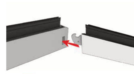
8 Loosen pre-fixed top bracket screw and slide hip rafter and top bracket into slot provided in the ridge body.
