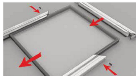
7 Fit glazed unit into the sash frame and re-fit the removed side of the sash framework, securing with the grub screws.
